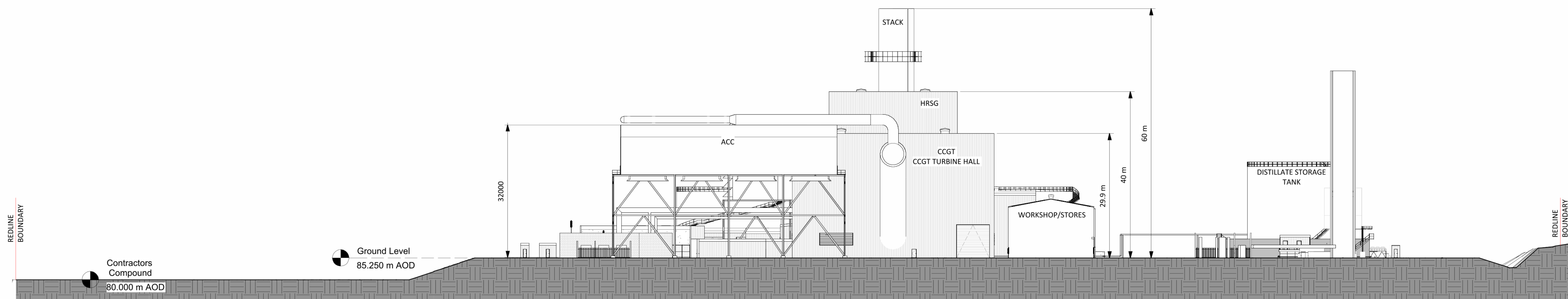
1 Main Site North South Section A-A 1 : 500
