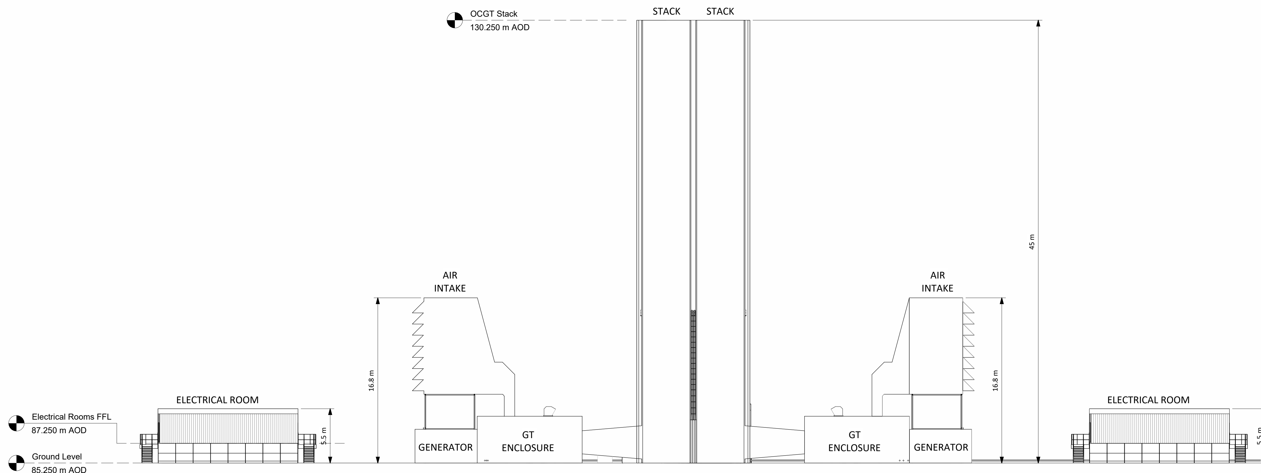
1 Section A-A Through OCGT 1 : 200
